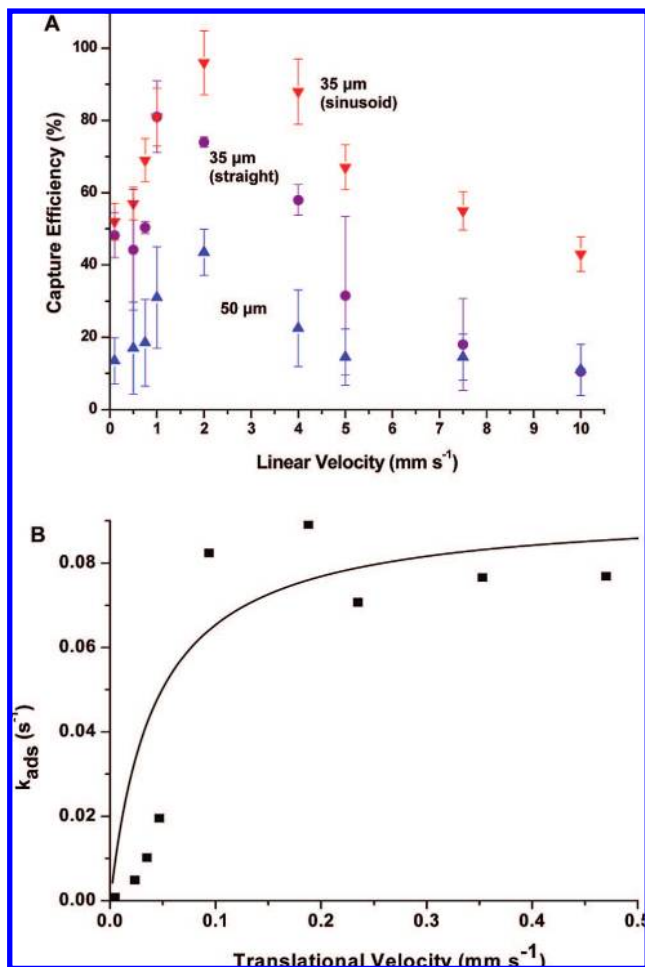
Figure 3. Data showing the capture efficiency of CTCs in spiked whole blood samples as a function of the cells' translational velocity using 35 (red down triangles, sinusoid; purple circles, straight) and 50 \mu\text{m} (blue up triangles) wide microchannels. (A) The microfluidic device consisted of a single channel with the appropriate width and a depth of 150 \mu\text{m} . Following processing of the input buffer containing the MCF-7 cells, the number of captured cells was determined via brightfield microscopy by interrogating the entire length of the capturing channel. (B) The capture efficiency data as a function of the CTC translational velocity were replotted using eq S16 (see Supporting Information) with this data fit to K_f \times C_x \times N_f using the fitting parameter, k_{in} (EpCAM/anti-EpCAM forward rate constant).
